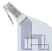
Y-Adapter RJ45m-2xRJ45f/s
