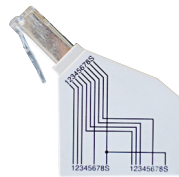
Adaptateur Y RJ45m-2x RJ45f/s
